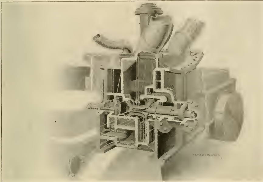
RICHMOND COMPOUND—INTERCEPTING VALVE IN COMPOUND POSITION.
